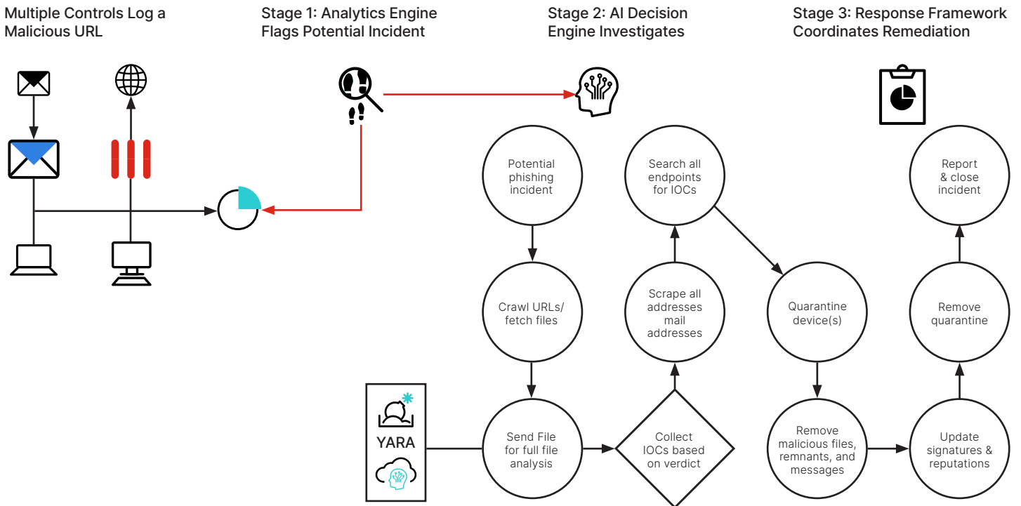
Figure 2: Phishing detection, investigation, and response.
